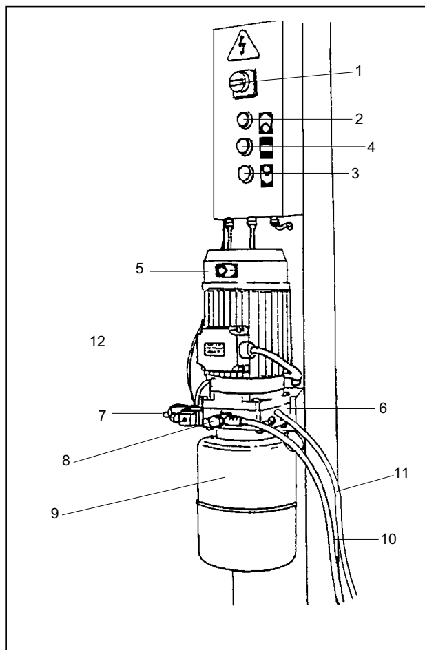
Fig.6 Control panel and hydraulic power unit.
