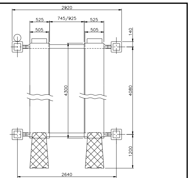
Fig.11a - Overall dimensions and clearances with platforms without recess for wheel alignment
