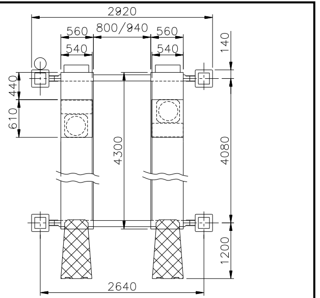
Fig.11 - Overall dimensions and clearances with platforms for wheel alignment
